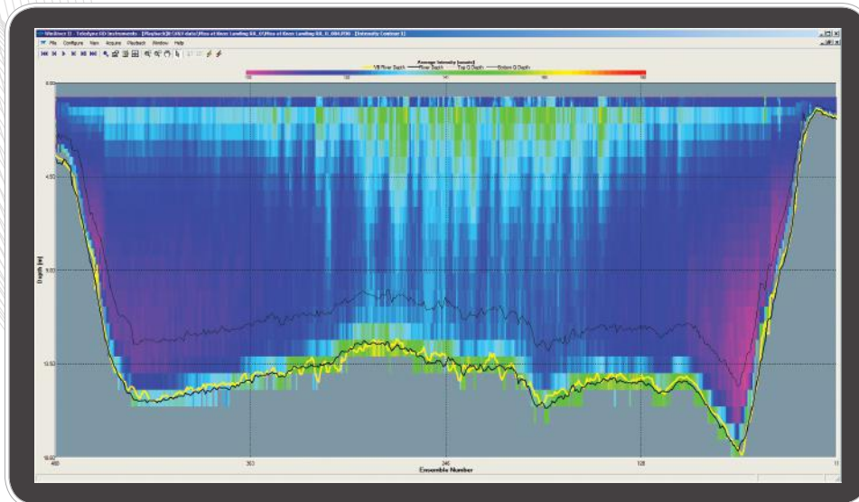
Sample RiverRay ADCP data collected on the Mississippi River in Baton Rouge, LA.
