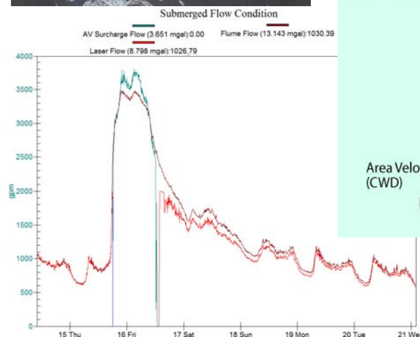
Figure 8: (Above) When water reaches the LaserFlow, the optional 350 area velocity sensor takes over flow rate measurement.
